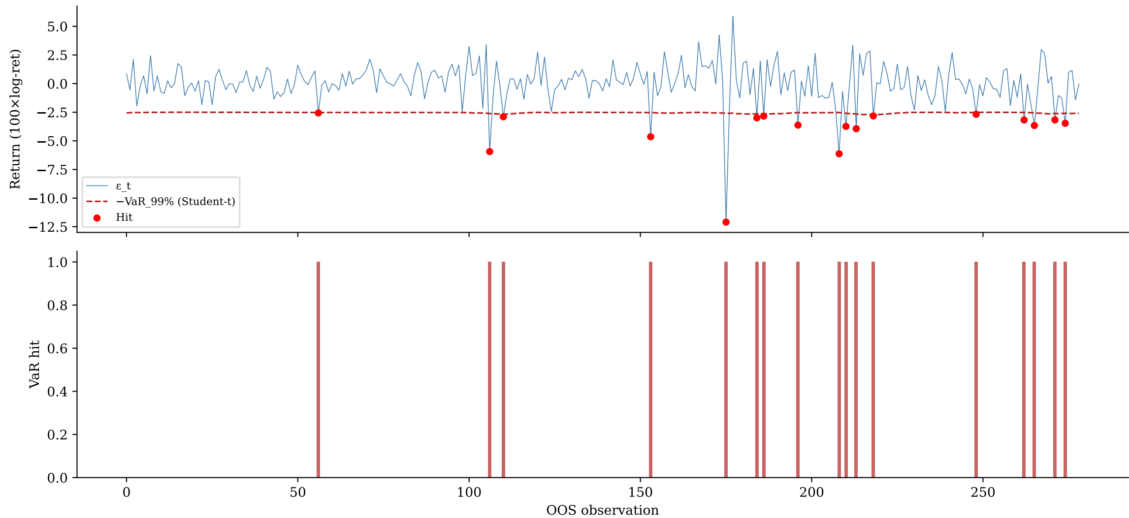
LSTM-SSE-t-Student — GOLD VaR 99% Hit Sequence
